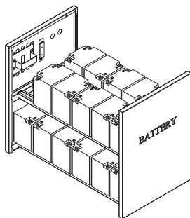
22pcs Batteries 33AH 196 × 131 × 156 (L × W × H)
