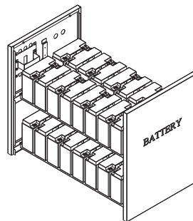
32pcs Batteries 15AH/20AH/22AH 181 × 77 × 167 (L × W × H)
