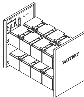
16pcs Batteries 38AH/45AH 198 × 166 × 170 (L × W × H)
