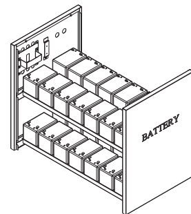
28pcs Batteries 12AH 151 × 98 × 100 (L × W × H)
