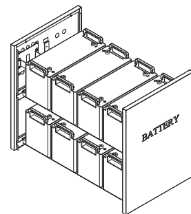
8pcs Batteries 100AH/120AH 407 × 174 × 236 (L × W × H)
