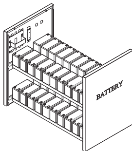
40pcs Batteries 6AH/7AH/9AH 151 × 65 × 100 (L × W × H)
